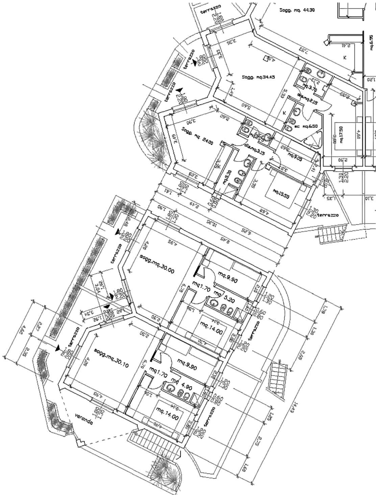
5 - Apartments Anemone in Palau: ground floor B
