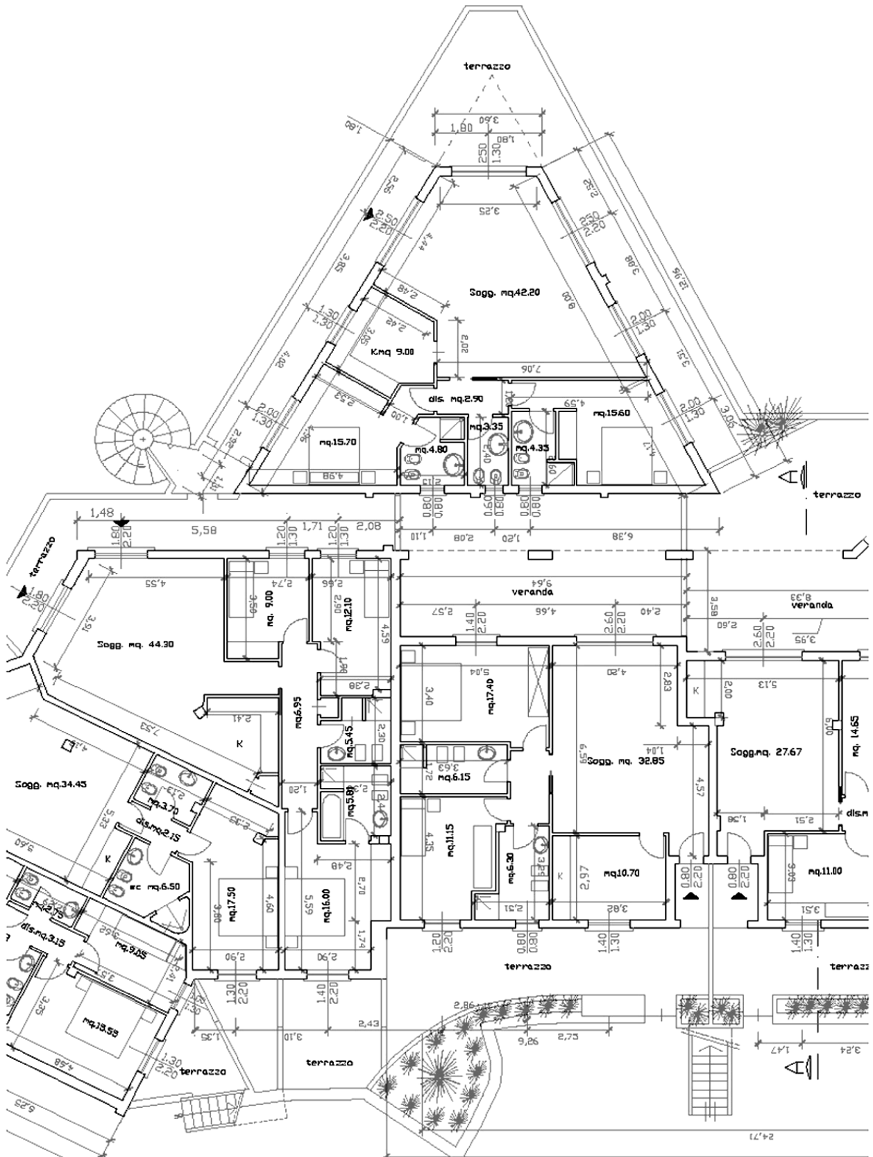
4 - Apartments Anemone in Palau : grond floor A
