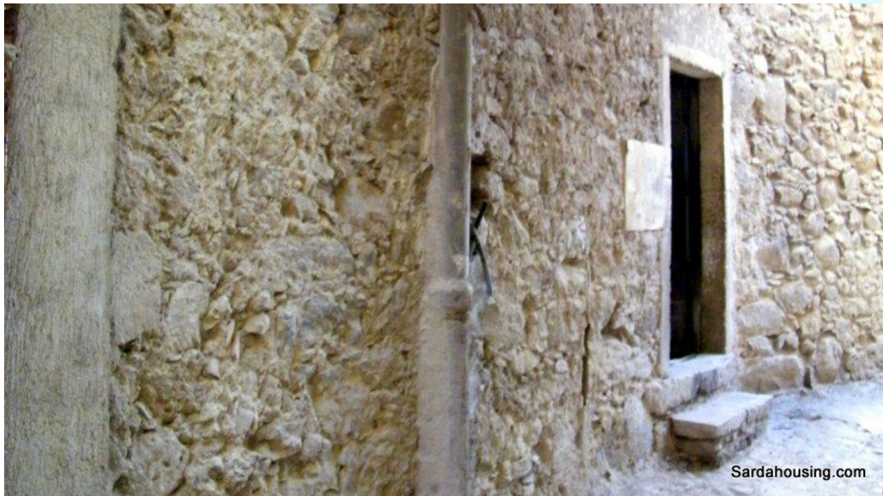
6 - Santu Lussurgiu – old centre - House La Volta: stone structure
